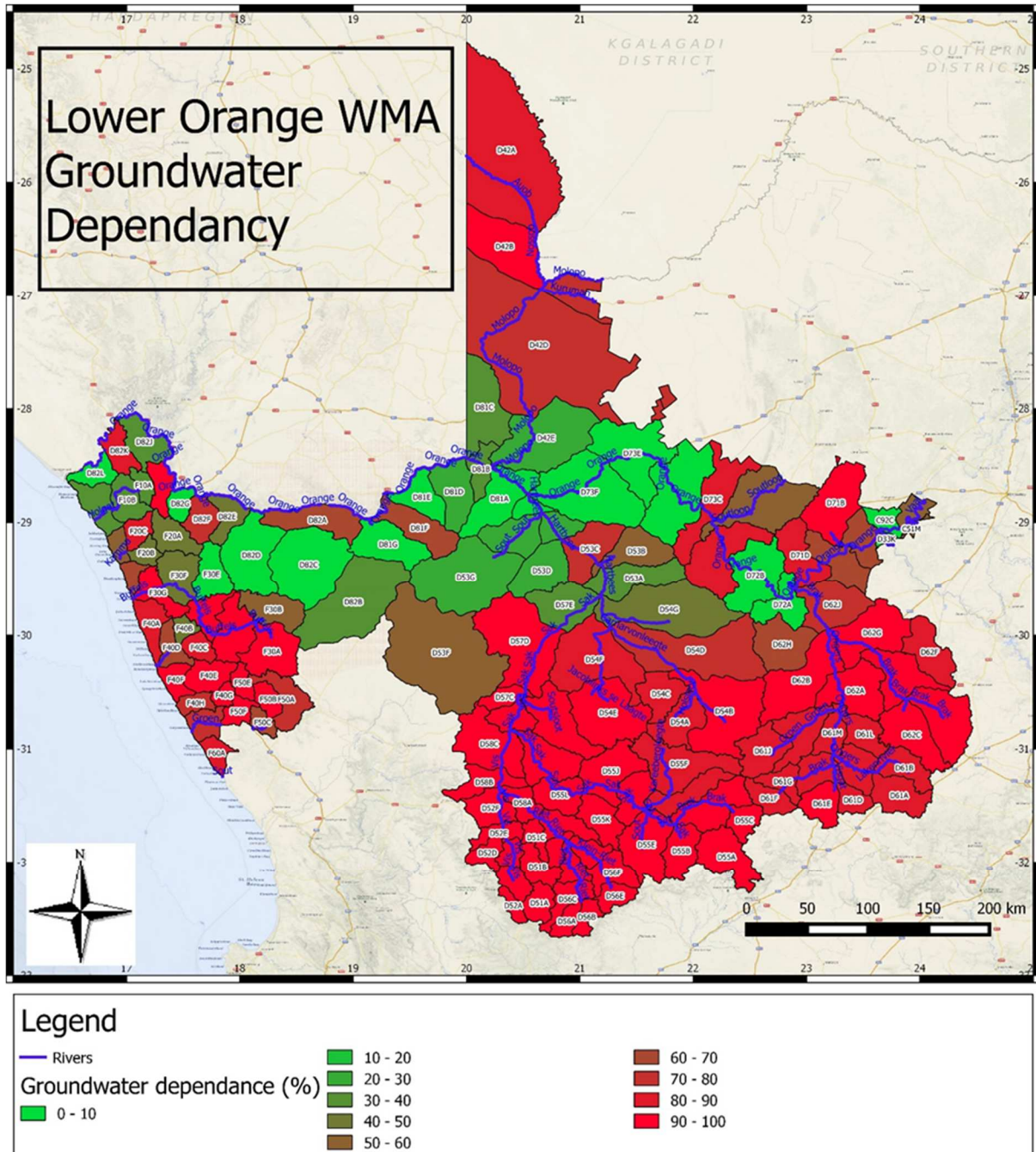
Figure 3-2 Groundwater Dependency
